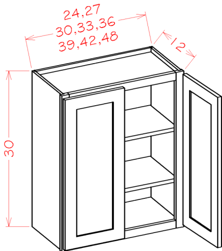
30" High Wall Cabinets - Double Door *2 adjustable Shelves
