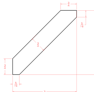
Crown Moulding - 3"H Angled Crown Moulding
